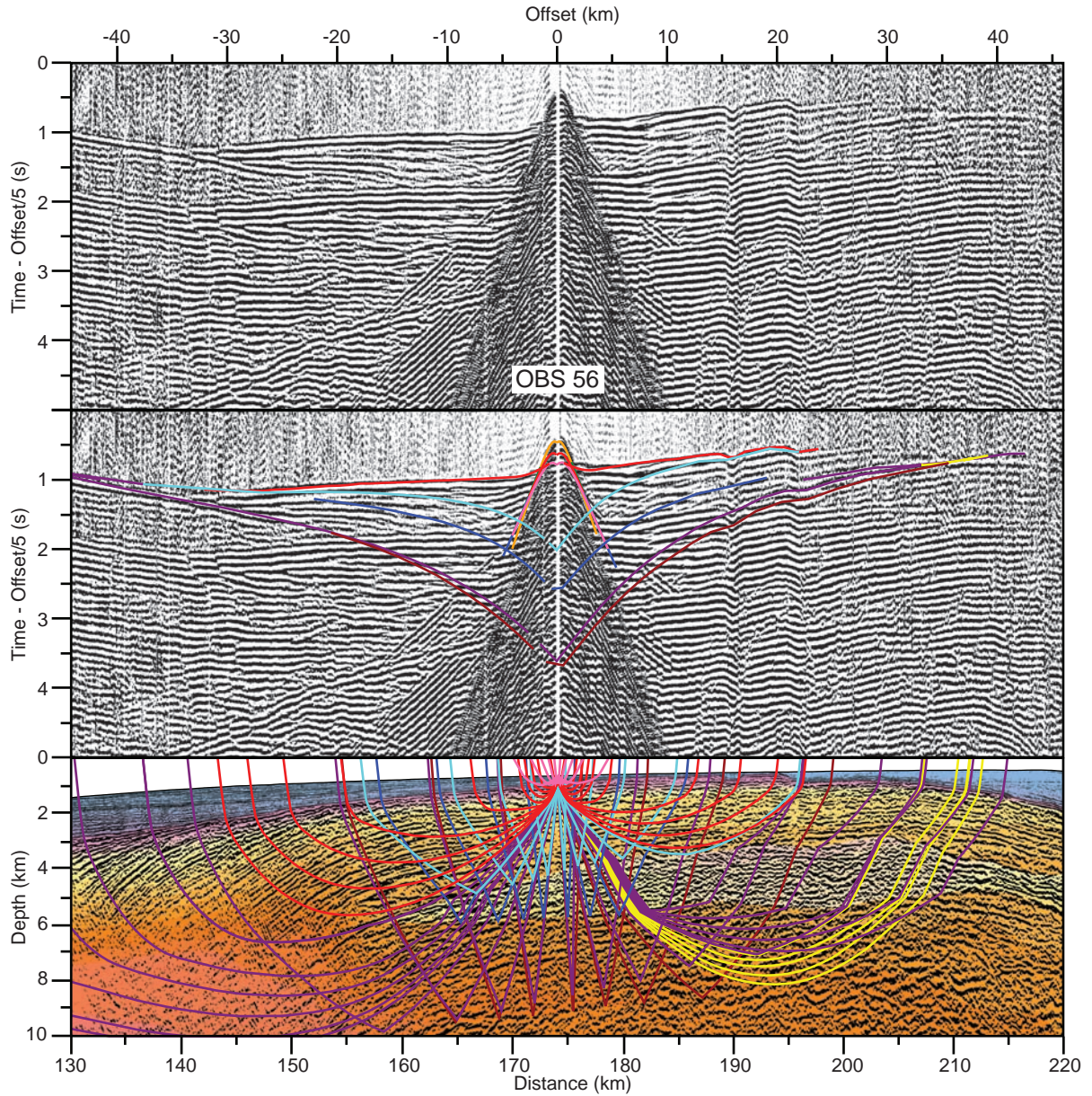
Fig S15. (Top) Record section for geophone data of OBS 56. A linear moveout at 5 km/s has been applied. Distances are measured from the north-northwestern end of the complete model (as in Roberts et al. 2009) and offsets are shot-receiver distances. (Middle) Record section with traveltime curves calculated by raytracing through the final velocity model and colour-coded by phases (see Figure 4 for legend). (Bottom) the corresponding ray path diagram with the same colour code as above. Only top basalt and deeper phases are shown for clarity. The seismic section was prestack depth migrated using the same final P-wave velocity model (colourmap) as is used in the raytracing. See text for modelling details. See Figure 8 in main paper for OBS location.
